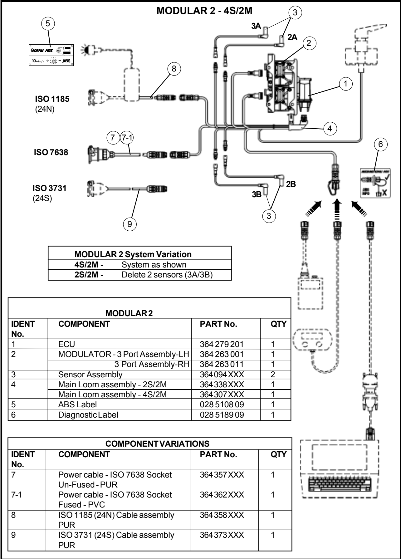
Fig 12.9 MODULAR 2 - 4S/2M WIRING VARIATIONS FOR SEMI TRAILER AND CENTRE
