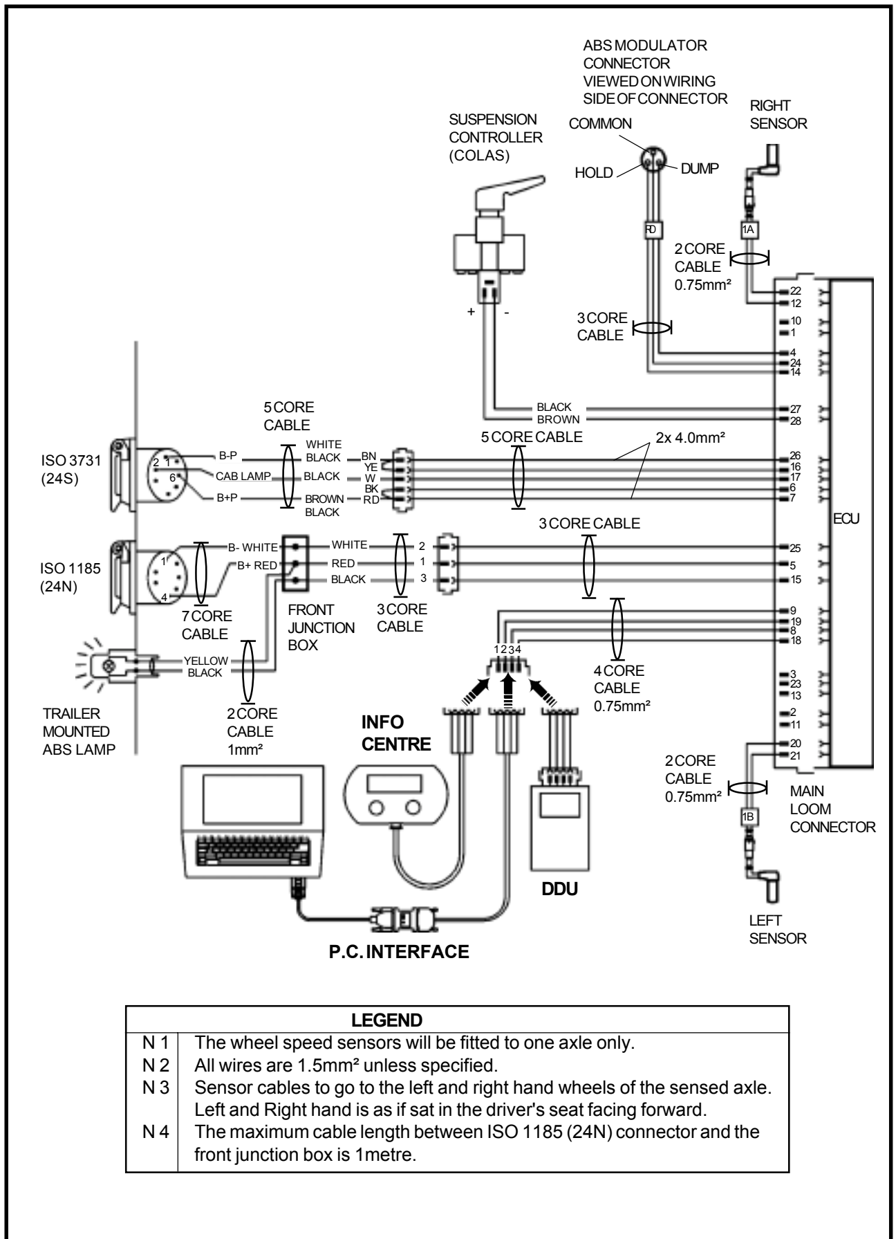
Fig 12.8 MODULAR 1 PLUS WIRING DIAGRAM ISO 3731 (24S) AND ISO 1185 (24N) POWER
