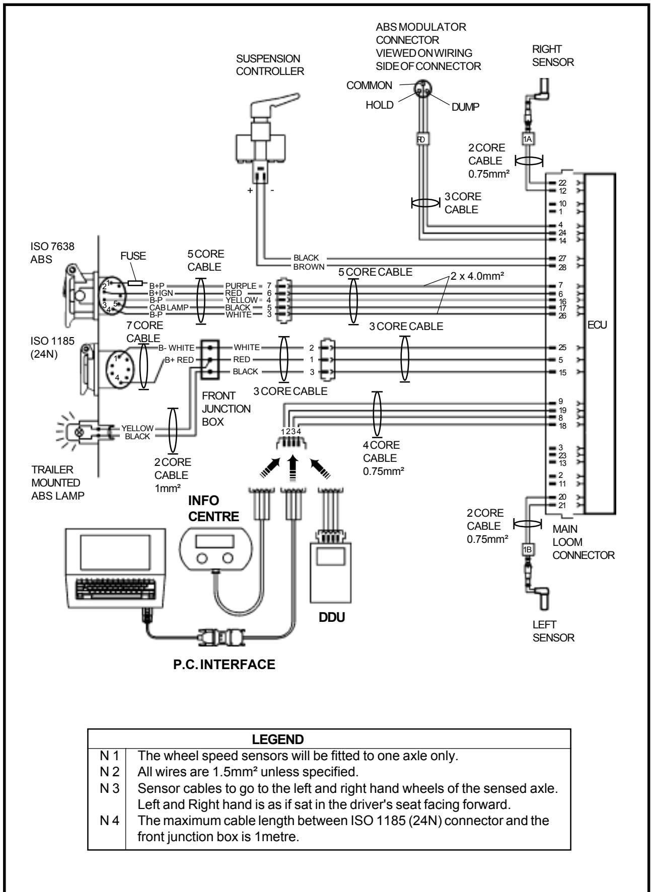
Fig 12.6 MODULAR 1 PLUS WIRING DIAGRAM ISO 7638 (FUSED) AND ISO 1185 (24N) POWER SUPPLY
