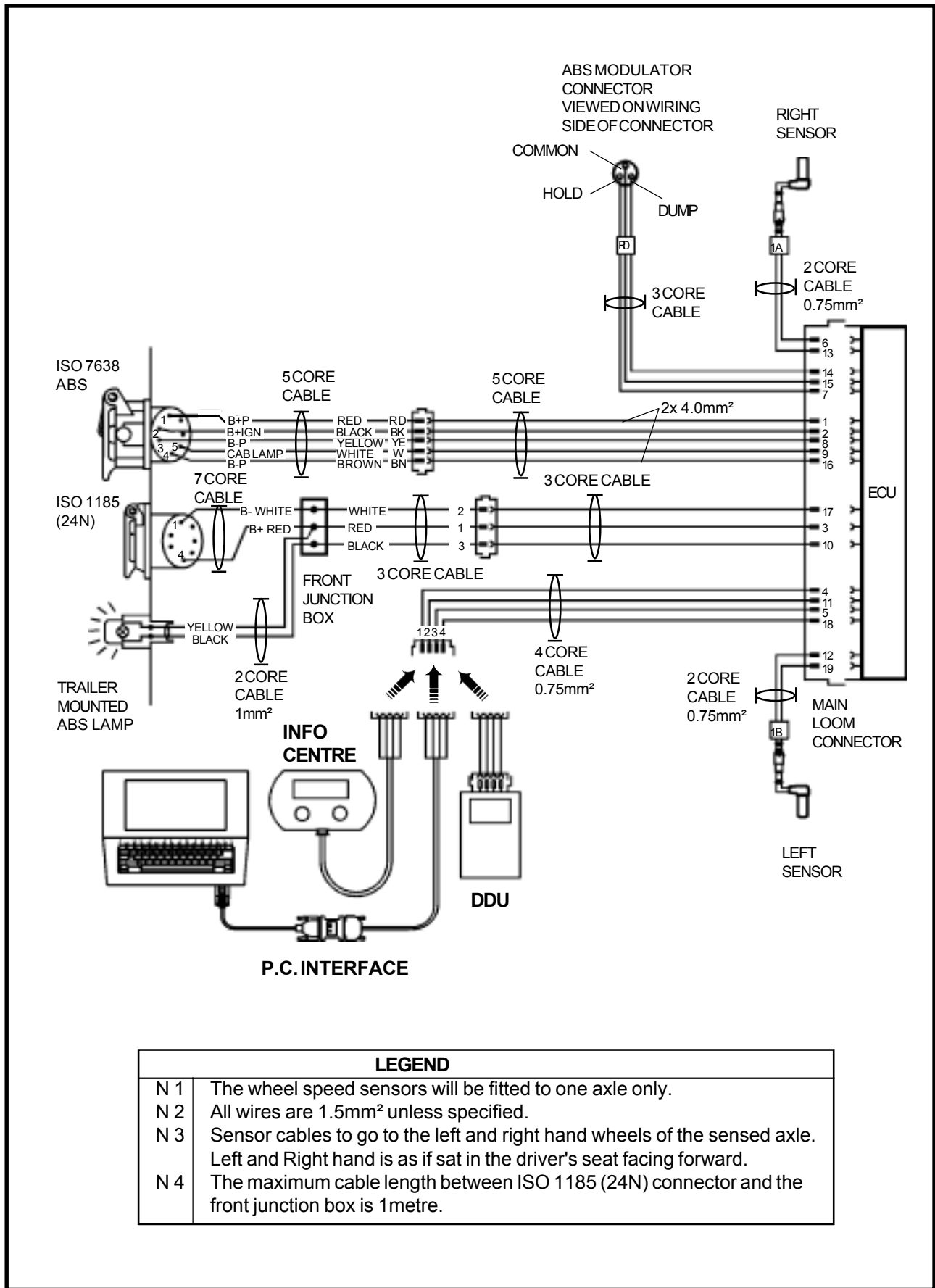
Fig 12.3 MODULAR 1 UPGRADE WIRING DIAGRAM ISO 7638 (UNFUSED) AND ISO 1185 (24N) POWER SUPPLY
