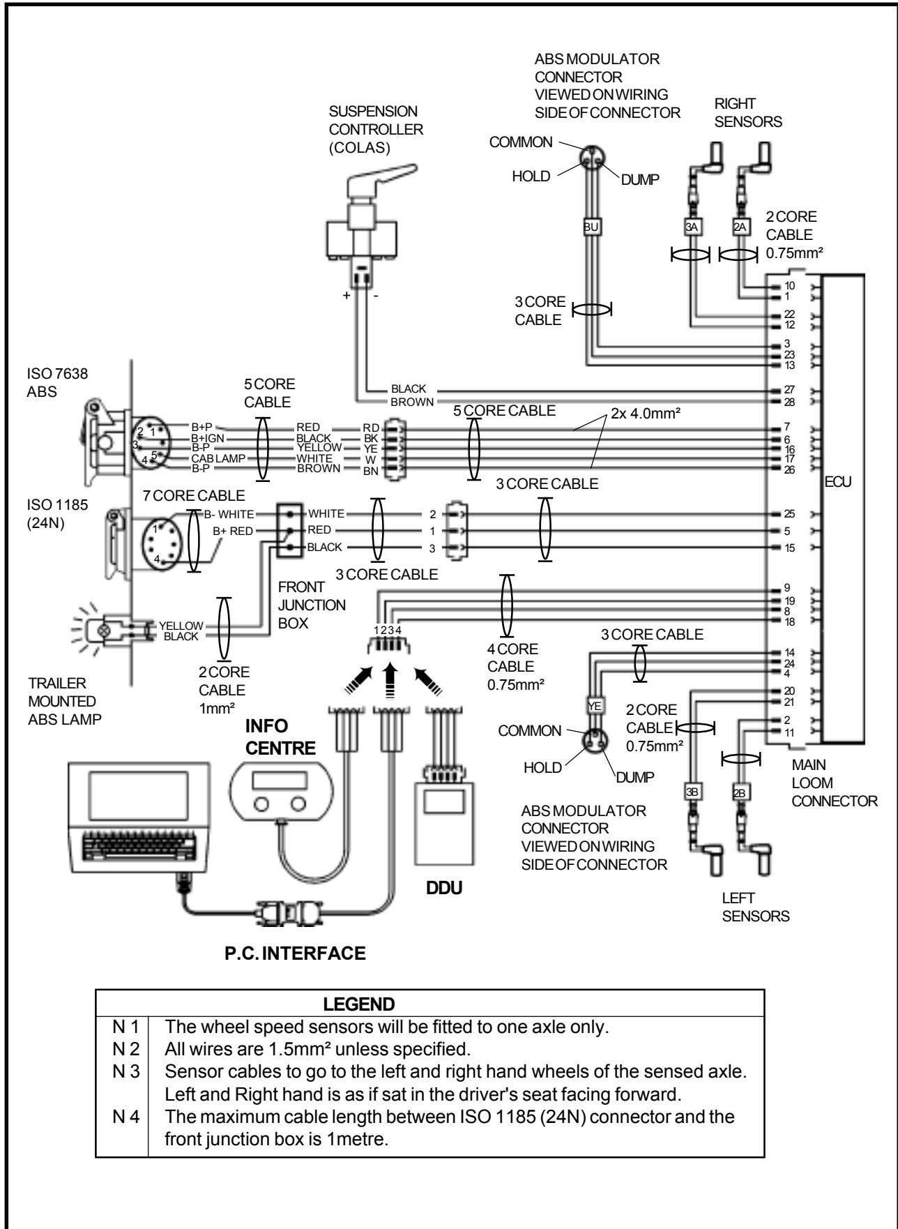
Fig 12.11 MODULAR 2 -4S/2M WIRING DIAGRAM ISO 7638 (UNFUSED) AND ISO 1185 (24N) POWER SUPPLY
