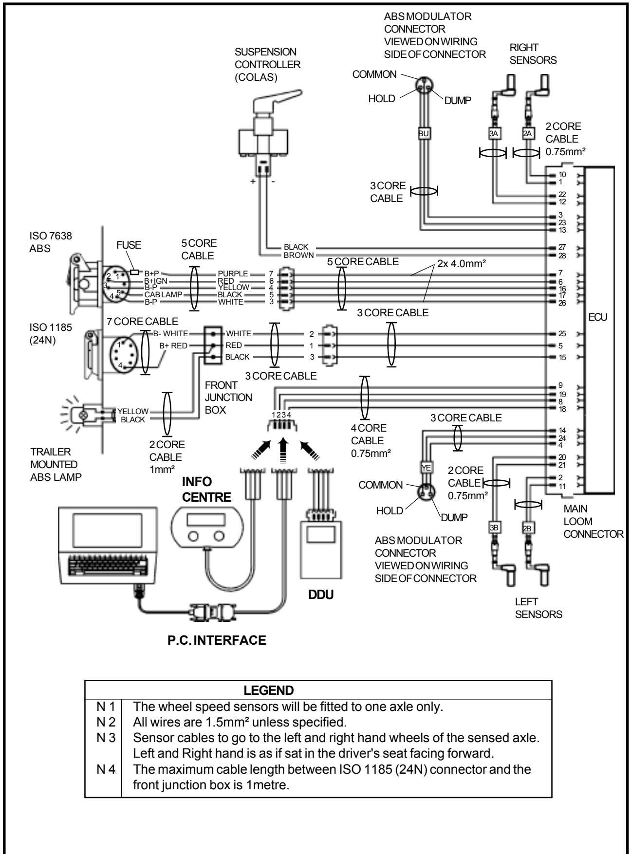
Fig 12.10 MODULAR 2 - 4S/2M WIRING DIAGRAM ISO 7638 (FUSED) AND ISO 1185 (24N) POWER SUPPLY
